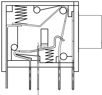
INTERNAL CONSTRUCTION
