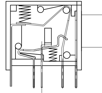
INTERNAL CONSTRUCTION
