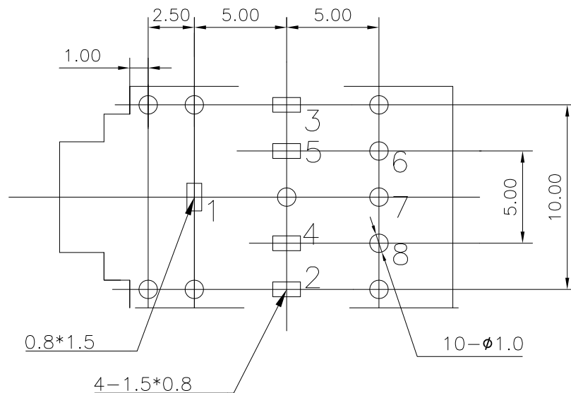
PCB LAYOUT TOP VIEW
