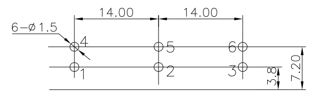
PCB LAYOUT TOP VIEW
